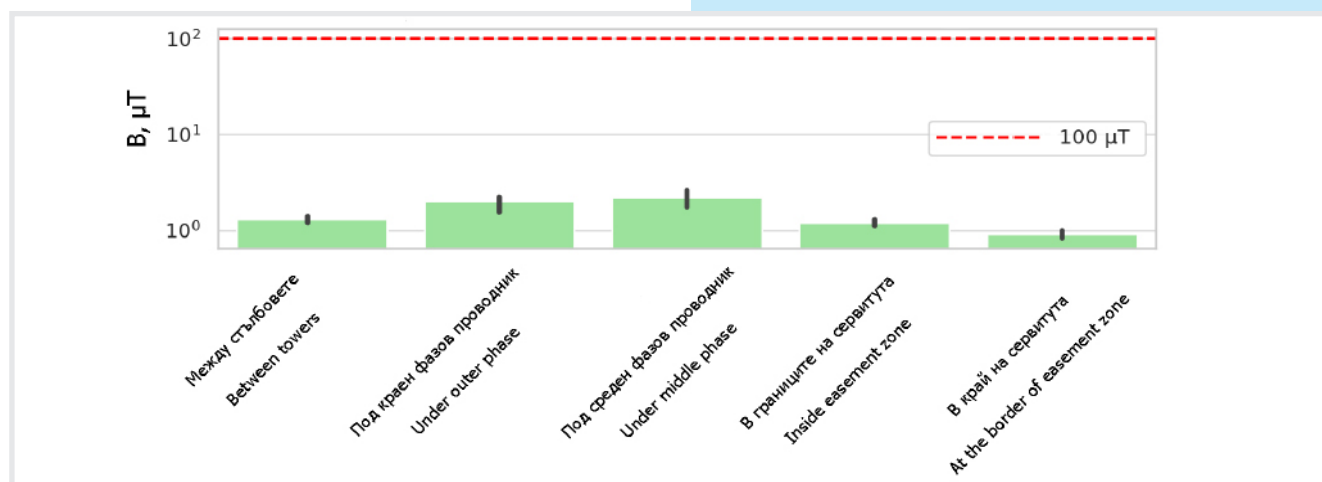
Figure 3. Magnetic flux density measured values compared the EU Council Recommendation 1999/519/EC
