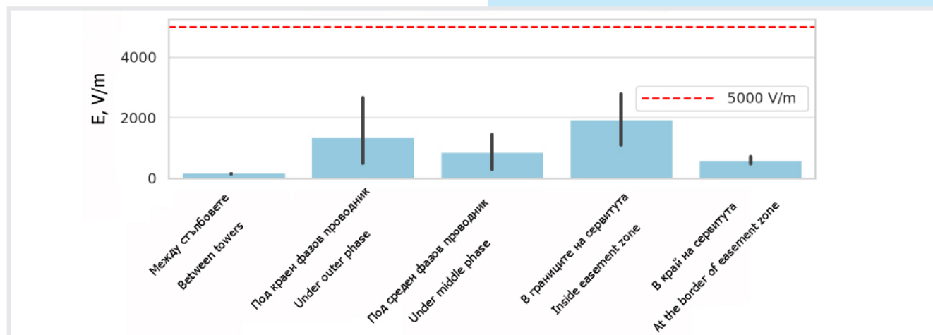
Figure 2. Electric field strength measured values compared to the EU Council Recommendation 1999/519/EC
